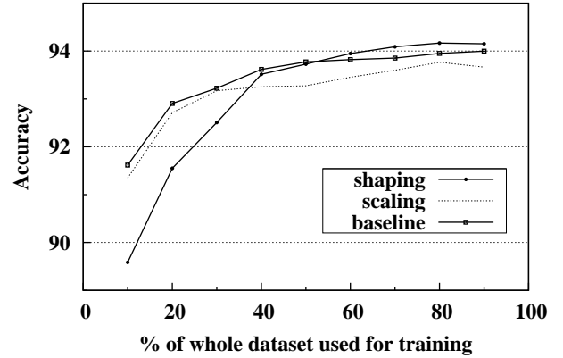
Figure 5: Accuracy learning curves for UCI.
