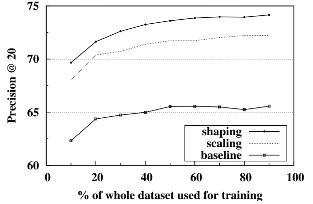
Figure 4: Precision@20 learning curves for UCI.
