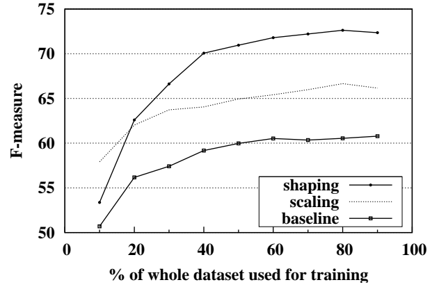
Figure 10: F-measure learning curves for the UCI benchmark.
