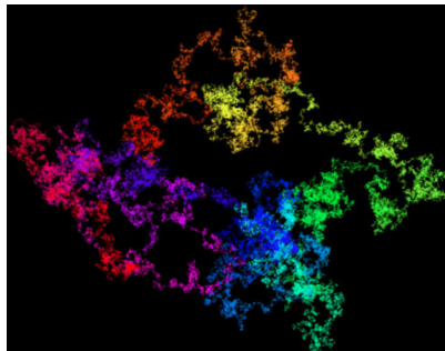
Fig. 2. A walk on the base-4 digits of \pi .
