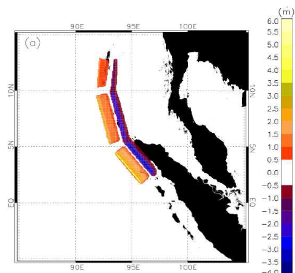
Figure 1. Location and magnitude of the sea floor displacement associated with the December 24 2004 tsunami. Taken from Greensdale et al. (2007)
